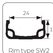
Rim type SW2 Black
