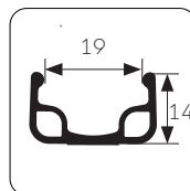
Rim type SW1 Silver or black aluminium
