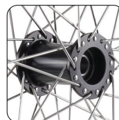
Hub type F1 black KTL steel hub, 49/59mm, 3 crosses
