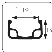
Rim type SW1 Silver coloured aluminium
