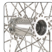
Hub type F2 alu hub 48/59mm. 36 stainless steel spokes. 3 crosses
