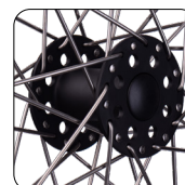
Hub type F5 High flange hub 53/64 mm, with 2,6 mm spokes and 3 crosses
