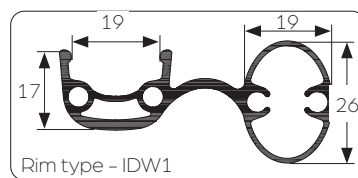
Integrated rim and pushrim in cast aluminium
